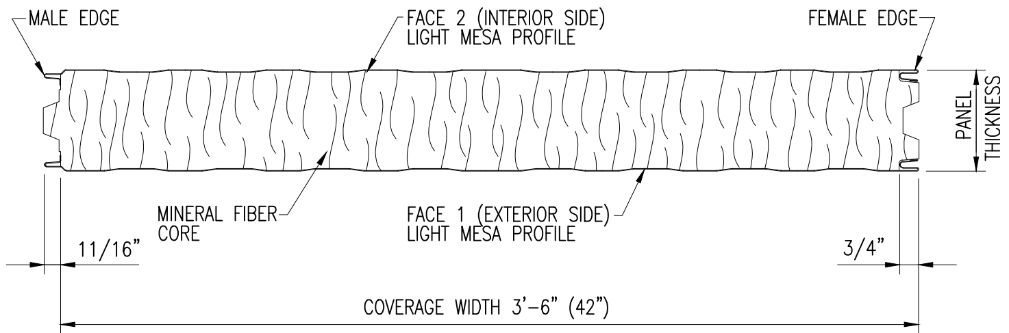
THERMSAFE ® FIRE RESISTANT PANEL CROSS SECTION
