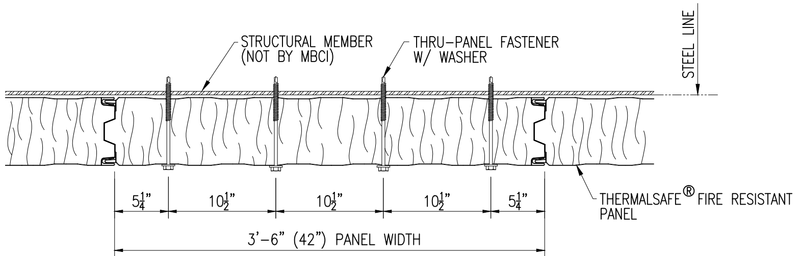
FASTENER PATTERN 2
