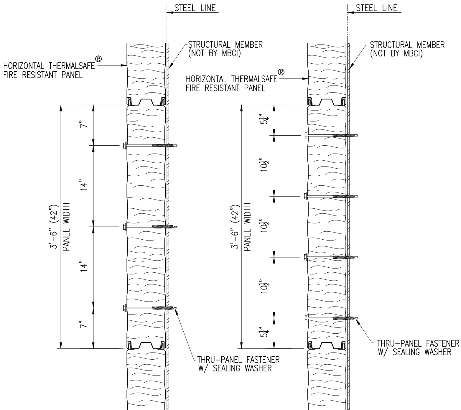
FASTENER PATTERN 1
