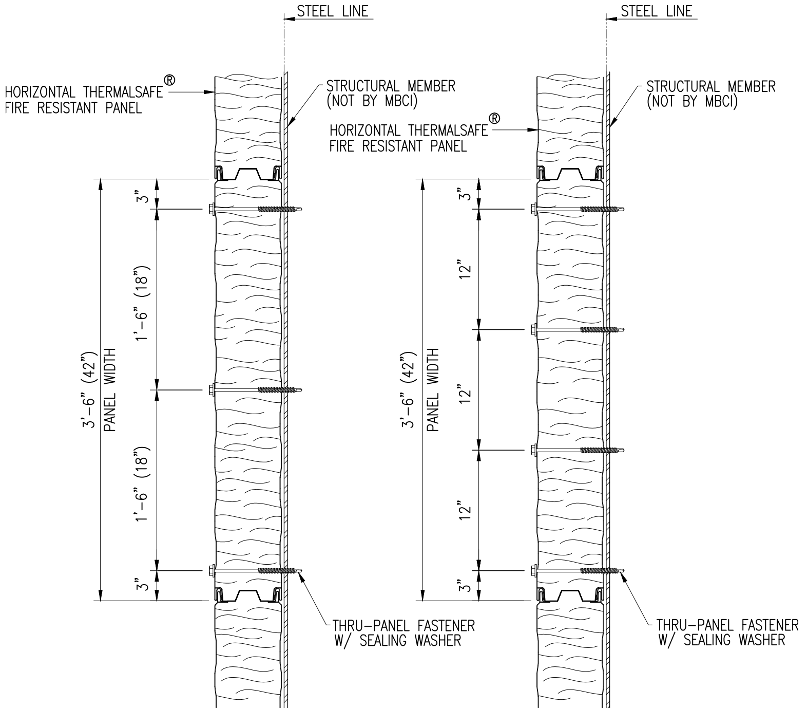
FASTENER PATTERN 1
