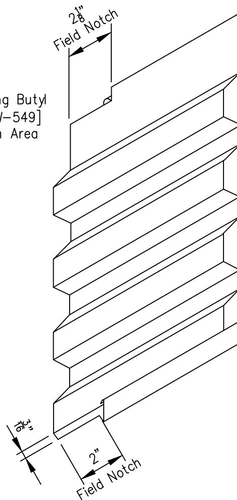
Panel Viewed From Interior Side
