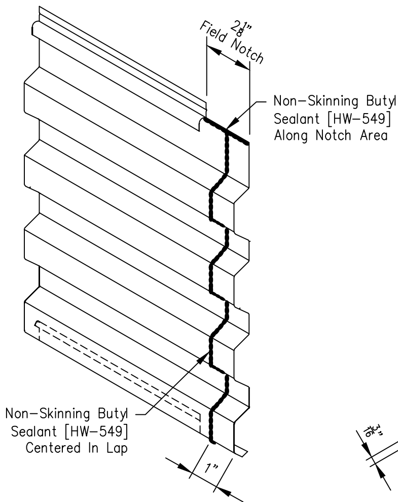
Panel Viewed From Exterior Side
