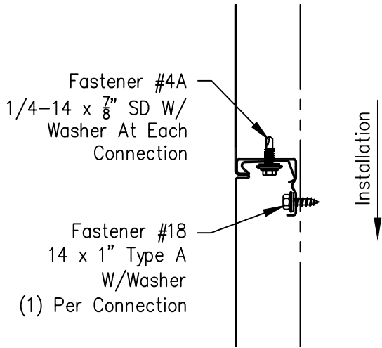
Side Lap - 12" Flat Panel
