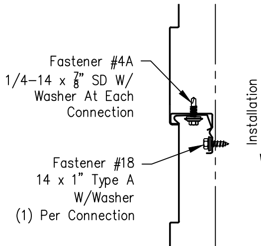
Side Lap - 16" Fluted Panel
