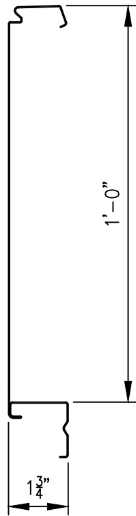
Designer Series Panel 12" Flat
