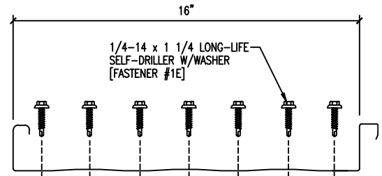
FASTENER LOCATIONS
