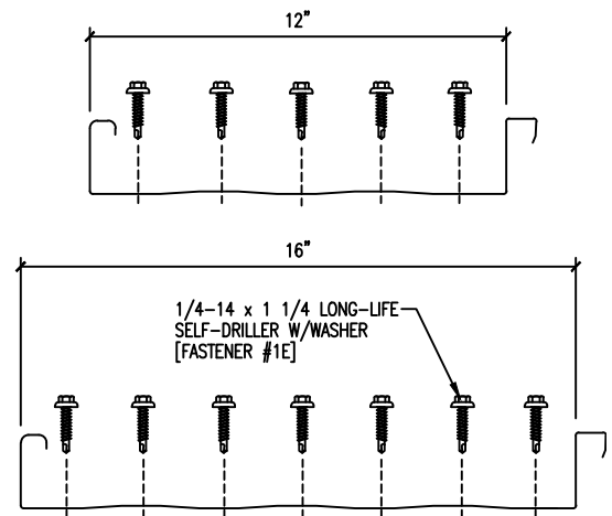
FASTENER LOCATIONS
