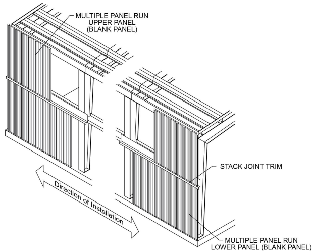
STACK JOINT WALL PANELS WITH TRIM PANELS MAY BE ERECTED FROM EITHER DIRECTION
