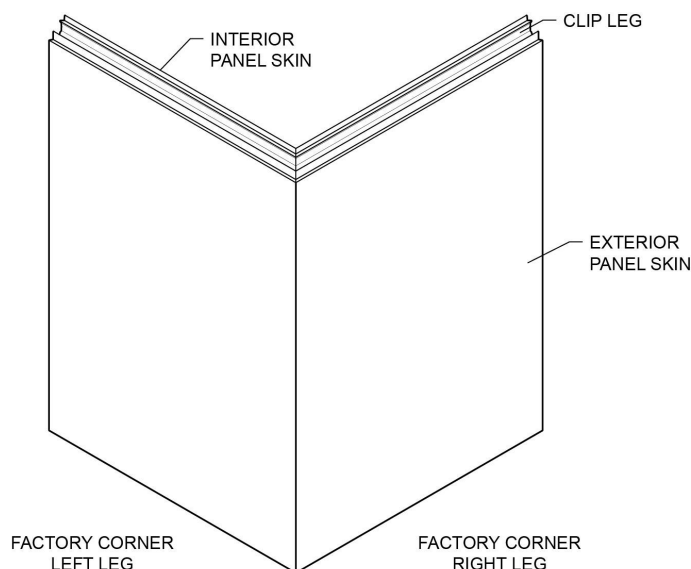
FACTORY FORMED OUTSIDE CORNER PANEL
