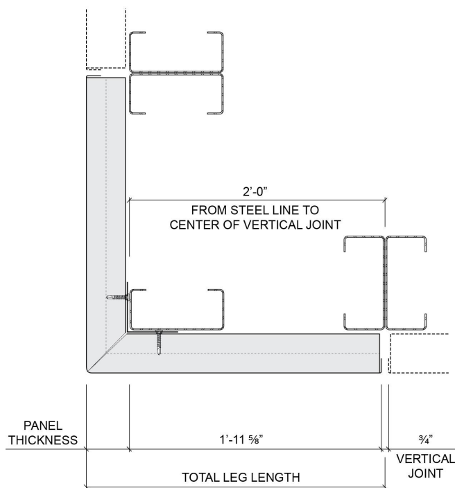
CALCULATING PANEL LENGTHS
