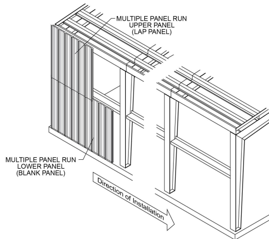
STACK JOINT WALL PANELS WITHOUT TRIM PANELS MUST BE ERECTED FROM LEFT TO RIGHT
